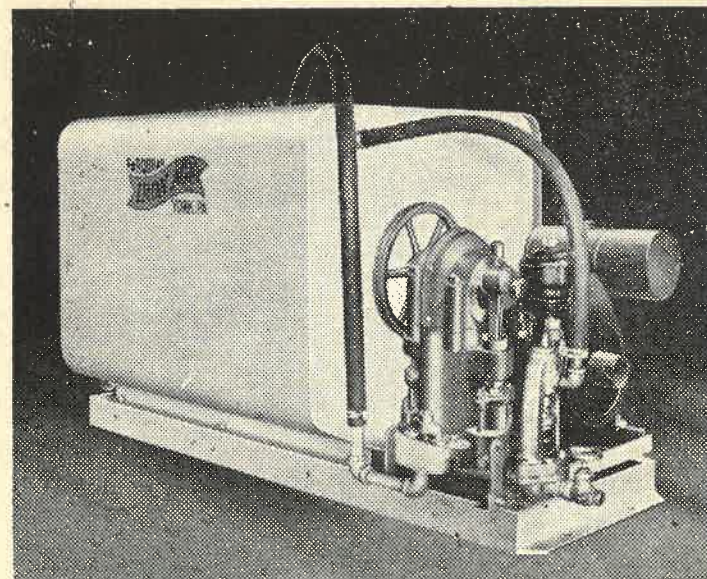
IRON AGE High Pressure SPRAYERS For Livestock
